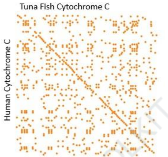
Figure 0.8 tuna fish vs Human
