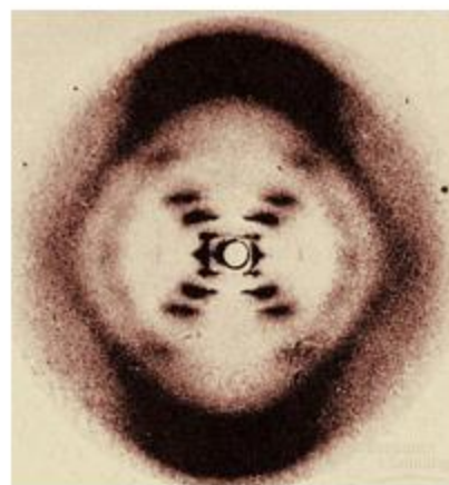
Rosalyn Franklin's Diffraction pattern for DNA
